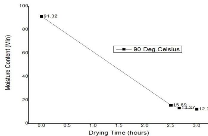
Graph 6: Deviations of Drying Time Vs Min. Moisture Content with Reference to Drying Temperature 90°Celsius
