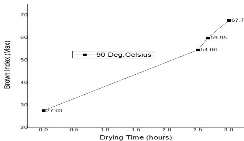
Graph 9: Deviations of Drying Time Vs Max. Brown Index with Reference to Drying Temperature 90°Celsius
