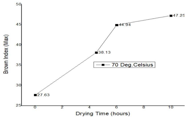
Graph 8: Deviations of Drying Time Vs Max. Brown Index with Reference to Drying Temperature 70°Celsius
