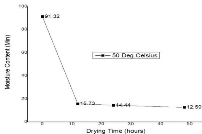
Graph 4 Deviations of Drying Time Vs Min. Moisture Content with Reference to Drying Temperature 50°Celsius
