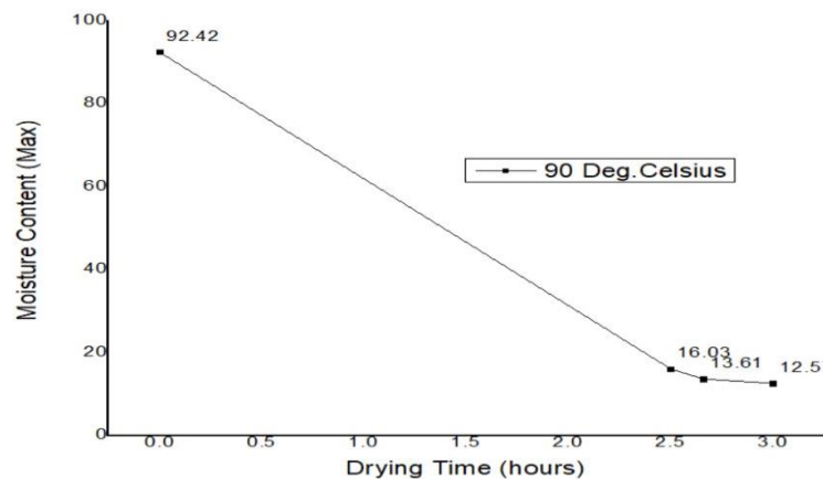
Graph 3 Deviations of Drying Time Vs Max .Moisture Content with Reference to Drying Temperature 90°Celsius
