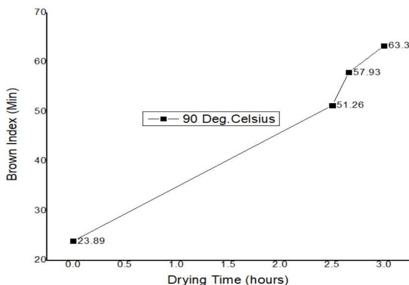
Graph 12 Deviations of Drying Time Vs Min. Brown Index with Reference to Drying Temperature 90°Celsius.
