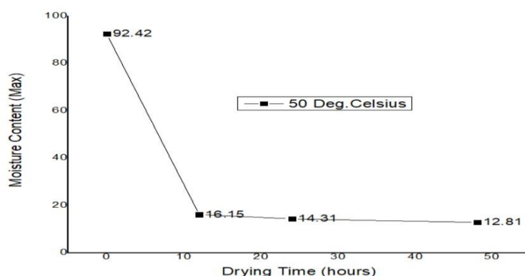
Graph 1: Deviations of Drying Time Vs Max. Moisture Content with Reference to Drying Temperature 50°Celsius
