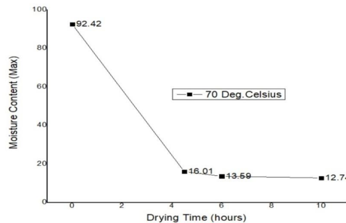
Graph 2: Deviations of Drying Time Vs Max .Moisture Content with Reference to Drying Temperature 70°Celsius
