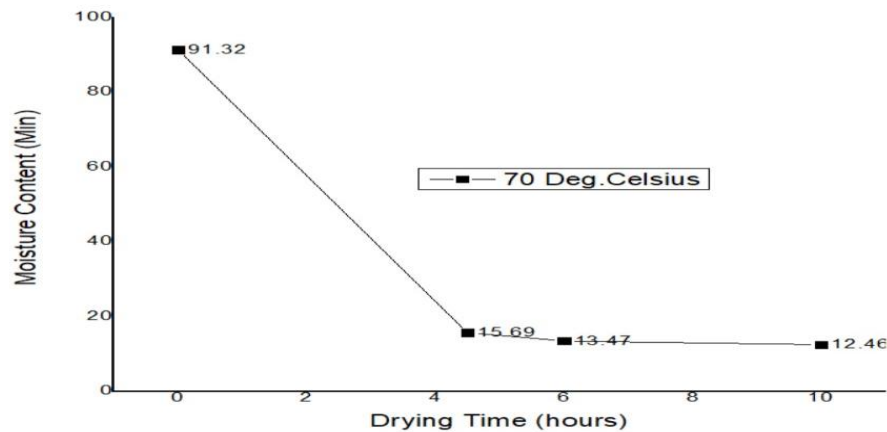
Graph 5: Deviations of Drying Time Vs Min. Moisture Content with Reference to Drying Temperature 70°Celsius
