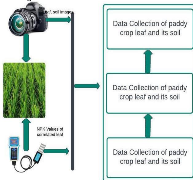
Figure 2. System architecture.
