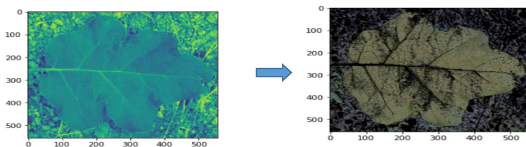
Figure 3. Data pre-processing.
